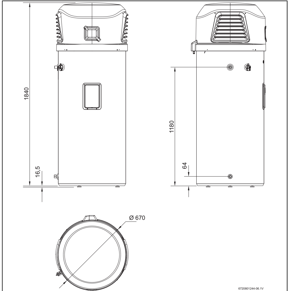
Fig. 6 Dimensions (in mm)
