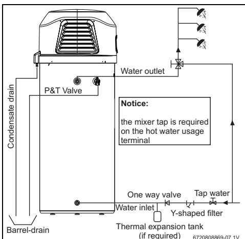
Fig. 9 Typical installation
