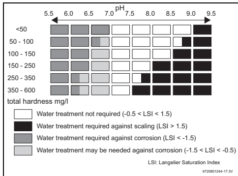
Fig. 18 Water treatment vs water characteristics
