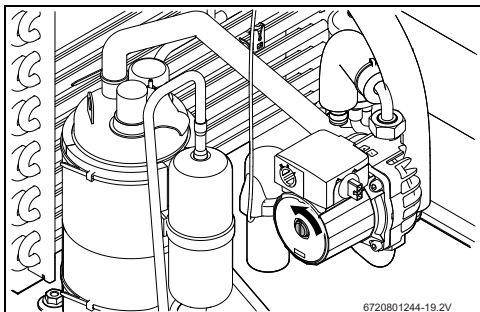
Fig. 17 Circulation pump purge screw
