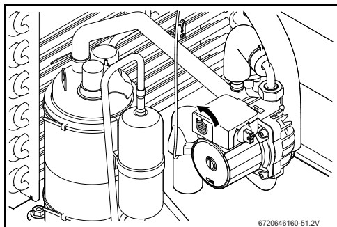
Fig. 15 Circulation pump
