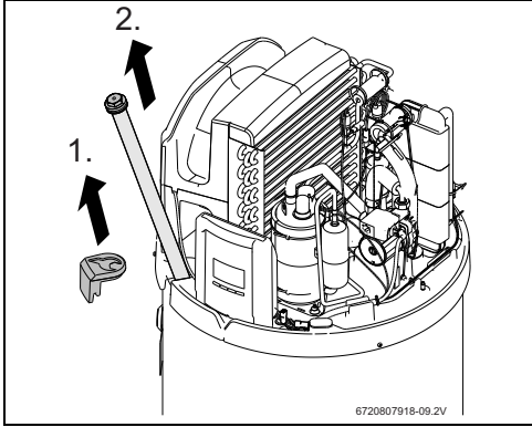
Fig. 60 Check state of magnesium anode
