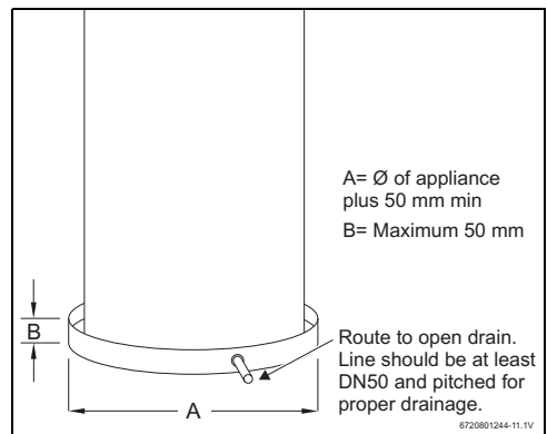
Fig. 8 Water heater support as specified in AS3500.4
