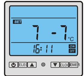
Parameter 7 Enter defrost mode Range: -30 to 0 deg C Default: -7 Adjustable by technicians
