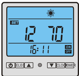
Parameter 12 Discharge temperature setting of compressor to close the solenoid valve Range: 60 to 80 deg C Default: 70 Adjustable by technicians
