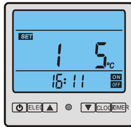
Parameter 1 Deadband temperature for re-heating Range: 2 to 15 deg C Default: 8 Adjustable by technicians
