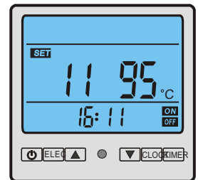
Parameter 11 Discharge temperature setting of compressor to open the solenoid valve Range: 70 to 120 deg C Default: 95 deg C Adjustable by technicians
