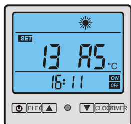
Parameter 13 Enter over temperature compressor protection cut-out Range: 90 to 127 deg C Default: 105 Adjustable by technicians
