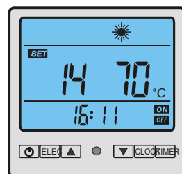
Parameter 14 Exit over temperature compressor protection cut-out Range: 60 to 80 deg C Default: 70 Adjustable by technicians
