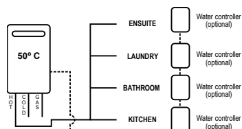
Diagram 1 - 50°C Appliance Minimum length of pipe from hot outlet to nearest hot water tap 2 metres.
